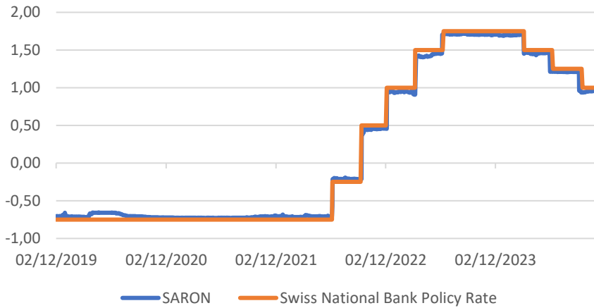
Andamento SARON Vs SNB Policy Rate
