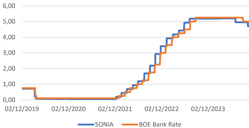
Andamento SONIA Vs BOE Bank Rate
