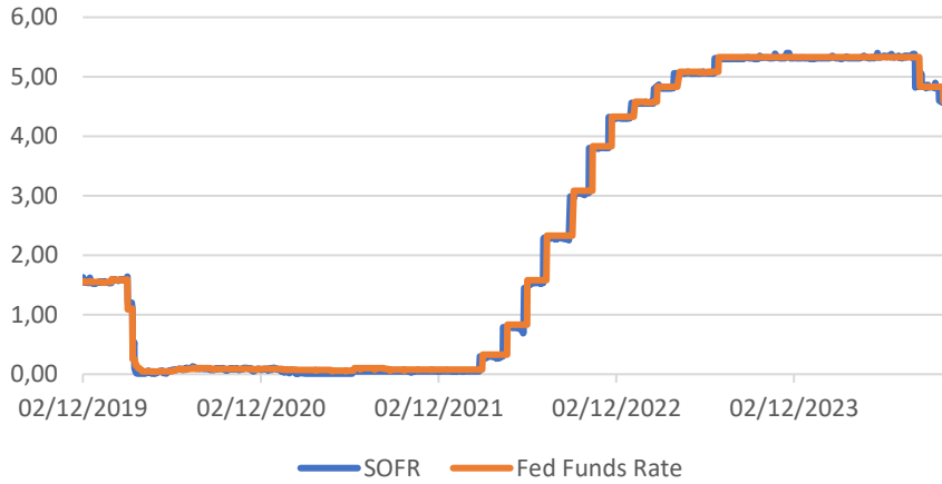
Andamento SOFR Vs Fed Funds Rate
